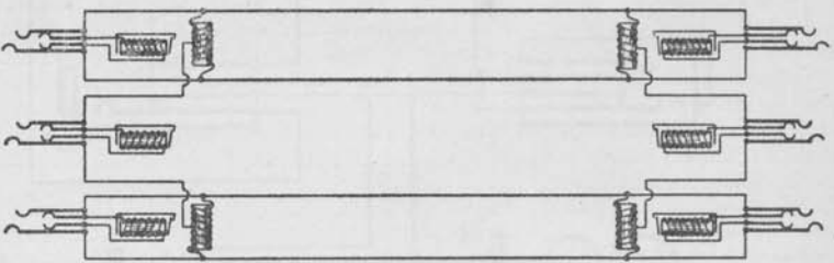
— FIG. 3 — — Metallic Phantom on Two Magneto Trunks —
