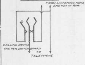
FIG 4 METHOD OF CONNECTING CALLING DEVICE
