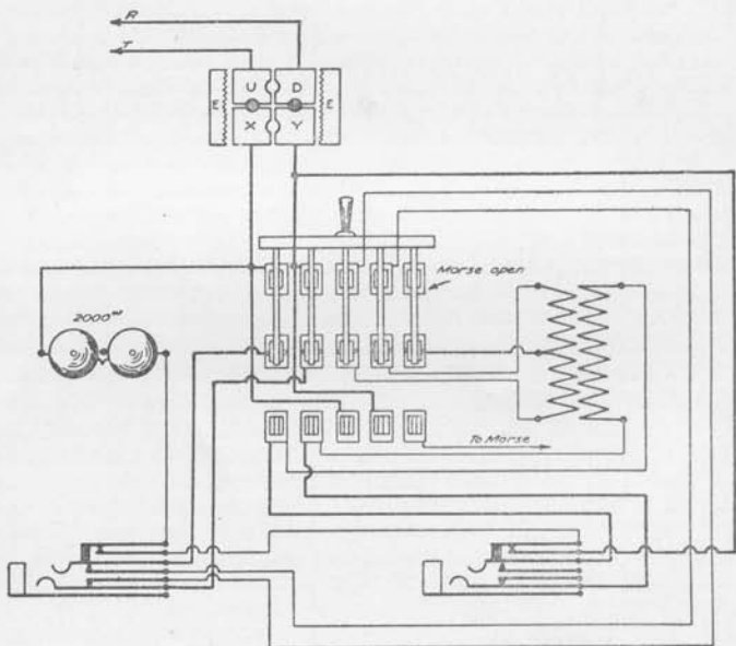
KNIFE SWITCH IN POSITION, METALLIC CIRCUIT, MORSE OPEN.
