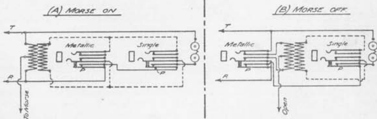
NOTE:— When a Plug is inserted in each of the Jacks, Contacts 'P' open.
