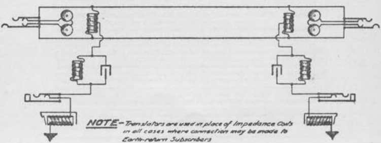
— FIG. 4 — — Earth-Return Phantom on a Magneto Trunk —
