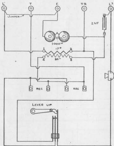
WIRING DIAGRAM
