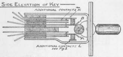
FIG 3 DETAILS OF CONTACTS L
