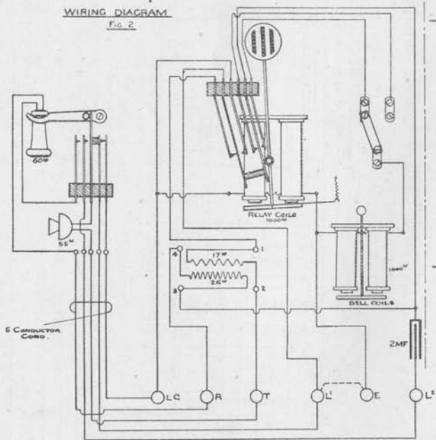
WIRING DIAGRAM
